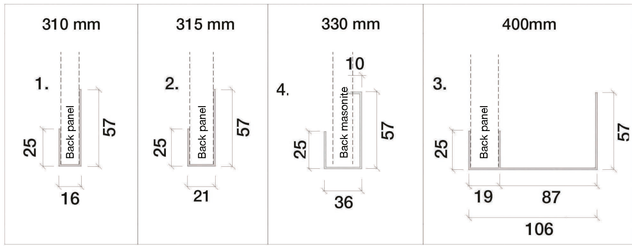
Compensator back hood detail for the back panel placement 4 different types of compensator according to wall unit depth:
